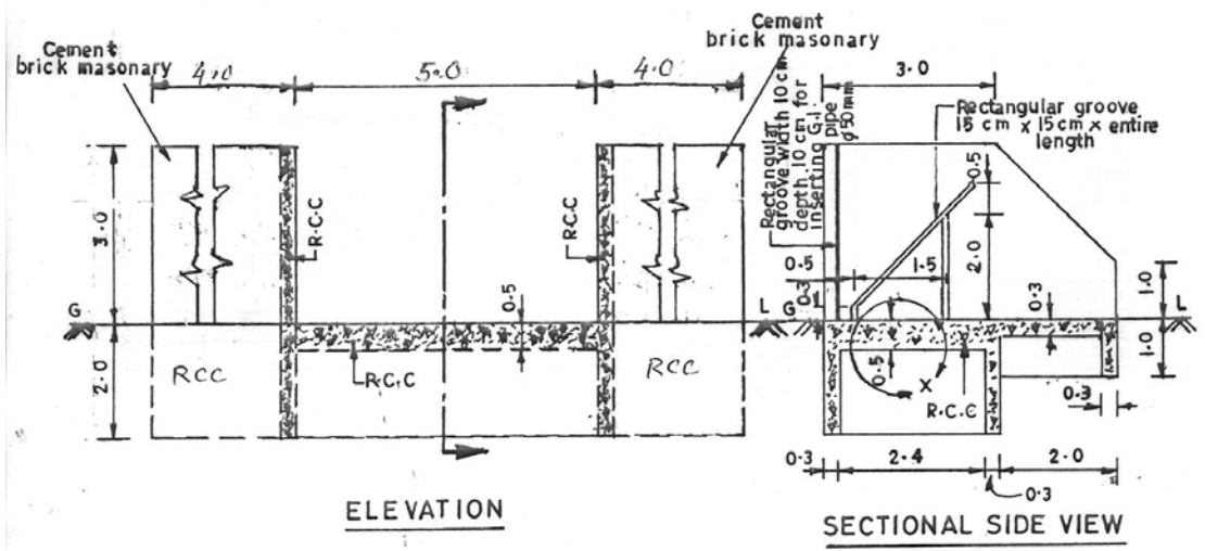
Rubberdam base structure at Sirsi, Jharkhand
